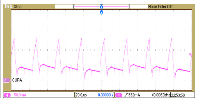
Figure 34. AutoTune
